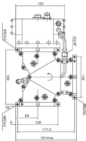
Outline Dimensions (mm(inch))
