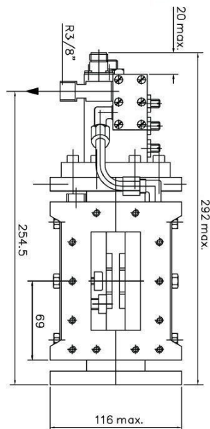
Outline Dimensions (mm(inch))
