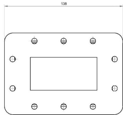
Outline Dimensions (mm(Inch))
